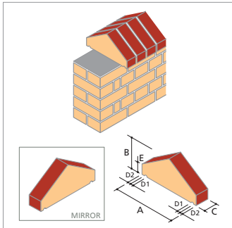
CP.2.1 Saddleback Copping
