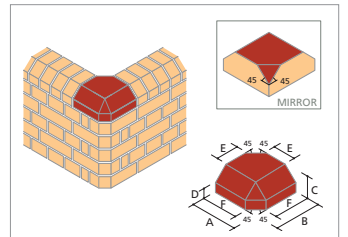
AN.17 Double Cant External Return With Internal Slope (Canted Corners On Bed)
