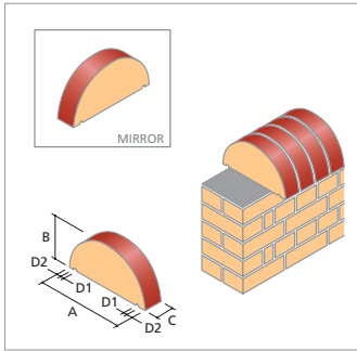
CP.1.1 Half Round Copping
