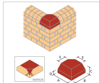
AN.16 Double Cant External Return With Internal Slope (Square Corner On Bed)
