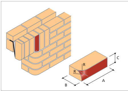
BN.7 Single Bullnose Internal Return Stretcher Faced (Left & Right Hand)
