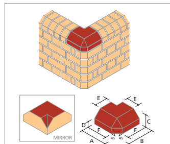
AN.15 Double Cant External Return With Internal Mitre (Canted Corner On Bed)
