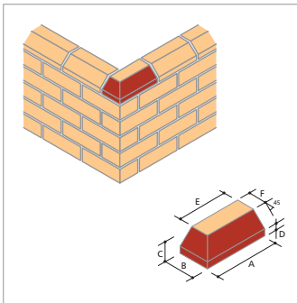
PL.5 Plinth Internal Return - short (Left & Right Hand)*
