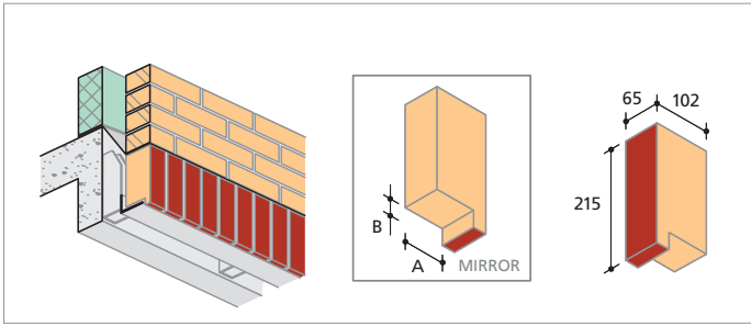
I.SA.1 Rebated Soldier
