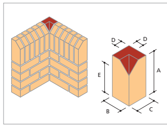
SD.2 Soldier Internal Return To Single Cant On End*
