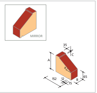
I.C.1 Overhanging Angled Sill
