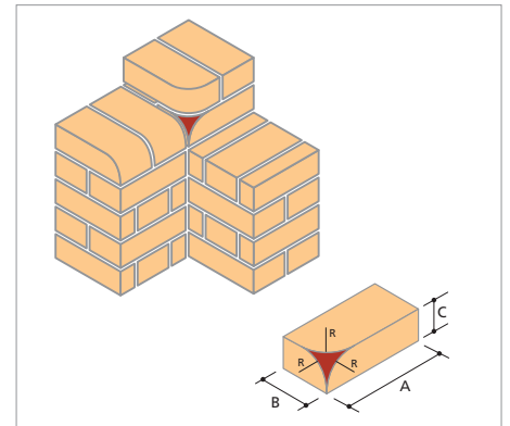
BN.12 Bullnose Mitre (Left & Right Hand)
