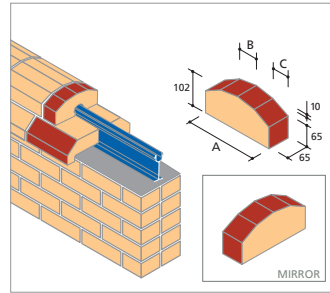
I.F.1 Faceted Copping †
