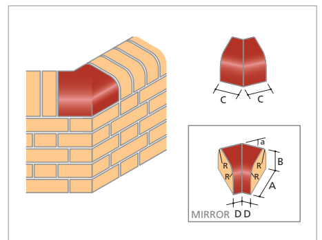
BN.21 Double Bullnose External Angle to Double Bullnose On Edge and to Bullnose Double Header On Flat
