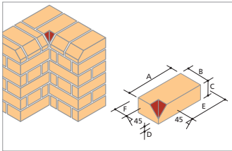
PL.5 Plinth Internal Return - short (Left & Right Hand)*
