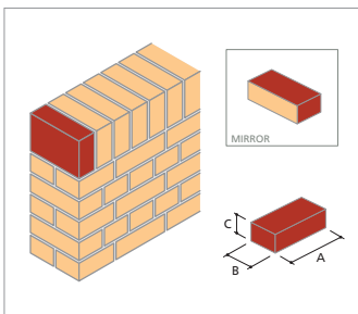
BD.1.3 Standard Brick fair-faced On Bed Surface
