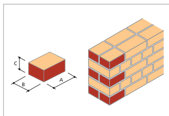
BD.1.2 Three-quarter Bat
