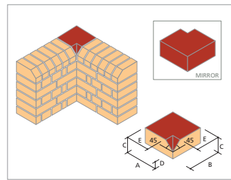
AN.8 Single Cant Internal Return With Internal Mitre (Square External Corner On Bed)
