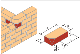
PL.1 Plinth Stop Or Cant Stop (Left & Right Hand)*
