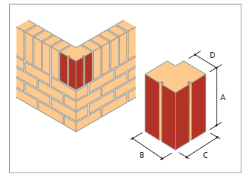
SD.1 Soldier External Return
