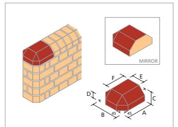
AN.13 Double Cant Stop End (Canted Corners On Bed)
