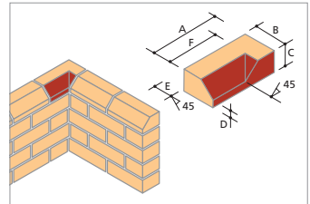
PL.4 Plinth Internal Return - long (Left & Right Hand)*
