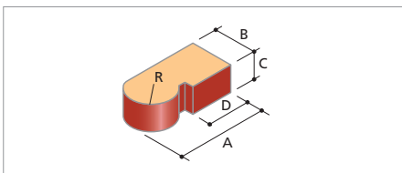
I.UJ.7 Easyangle® (Left & Right Hand)
