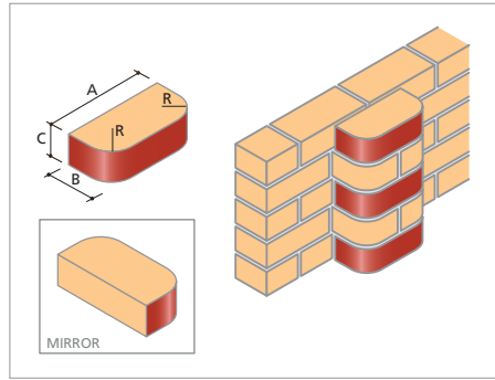
BN.2 Double Bullnose
