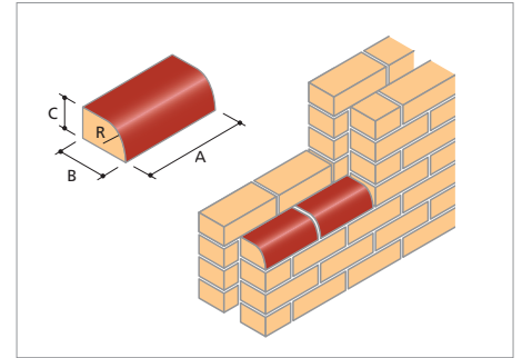
BN.6 Single Bullnose Stretcher On Flat
