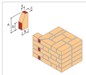
BD.2 King Closer
