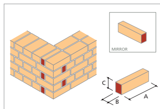
BD.3 Queen Closer
