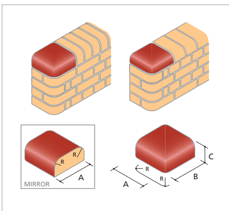
BN.18 Stop End to Double Bullnose On Edge and to Bullnose Double Header On Flat (Rounded Corners On Bed)
