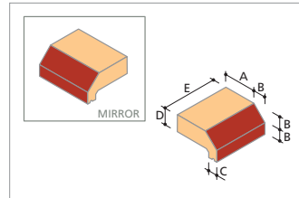
I.B.C.1 Base Copping Standard Brick**
