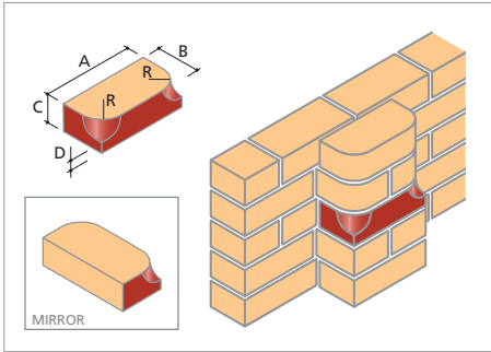
BN.4 Double Bullnose Stop
