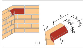
PL.6 Plinth Internal Angle (Left & Right Hand)*
