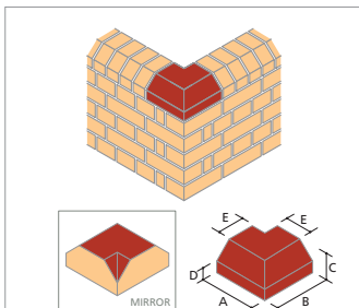
AN.14 Double Cant External Return With Internal Mitre (Square Corner On Bed)
