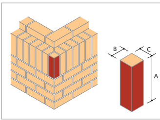
SD.1 Soldier External Return
