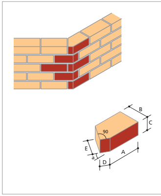
AN.1 Squint Brick (Left & Right Hand)
