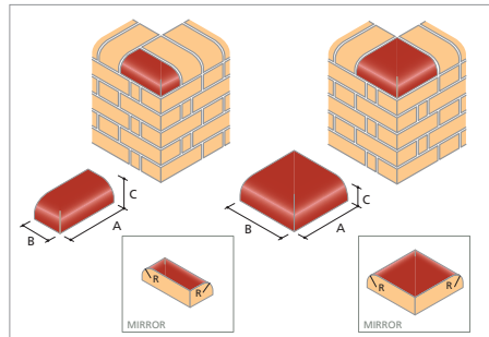
BN.11 Bullnose External Return On Flat (Left & Right Hand)
