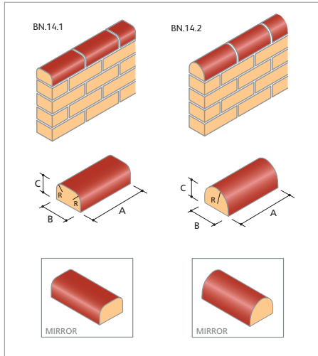
BN.14 Bullnose Double Stretcher On Flat
