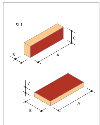
SL.1 Brick Face Slip
