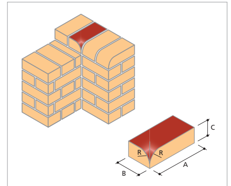
BN.9 Single Bullnose Internal Return Flat Faced (Left & Right Hand)
