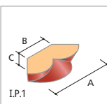
I.P.1 Pineapple Brick To 400mm Diameter Column
