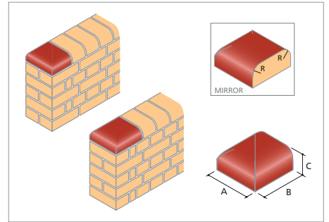
BN.15 Stop End to Double Bullnose On Edge and to Bullnose Double Header On Flat (Square Corners On Bed)
