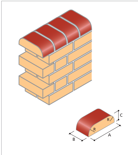
BN.13 Bullnose Double Header On Flat
