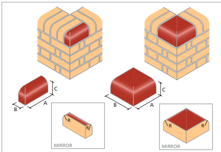
BN.10 Bullnose External Return On Edge (Left & Right Hand)
