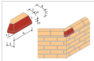
PL.9 Plinth Squint (Left & Right Hand)*
