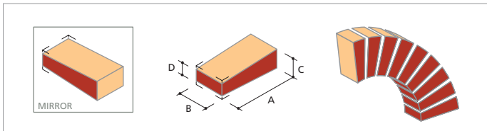
AR.2 Tapered Stretcher
