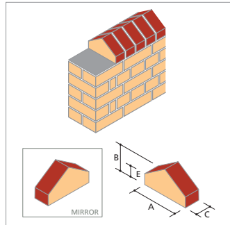
CP.2.2 Saddleback Copping
