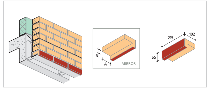
I.SA.4 Rebated Stretcher
