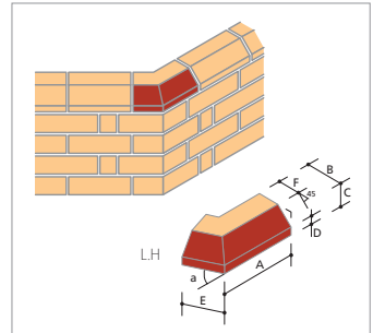
PL.8 Plinth External Angle (Left & Right Hand)*
