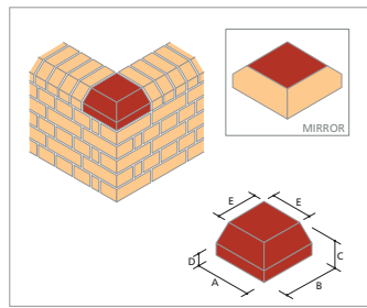
AN.7 Single Cant External Return
