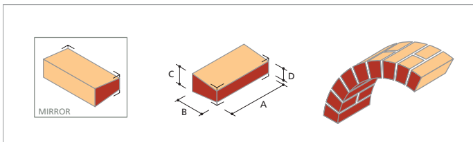
AR.1 Tapered Header
