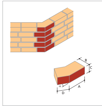
AN.2 External Angle (Left & Right Hand)
