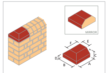
AN.12 Double Cant Stop End (Square Corners On Bed)
