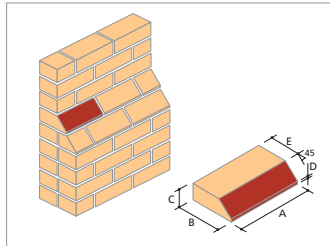
I.PL.15 Wide Bed Plinth Stretcher
