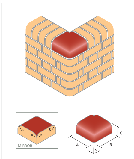
BN.20 External Return to Double Bullnose On Edge and to Bullnose Double Header On Flat (Rounded Corner On Bed)
