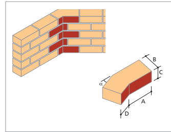
AN.3 Internal Angle (Dog Leg) (Left & Right Hand)
