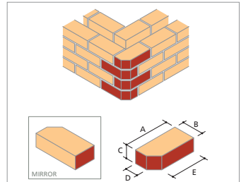
AN.5 Single Cant (Left & Right Hand)
