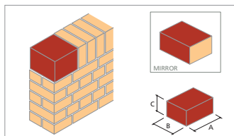
BD.4 215mm Square Stop End
