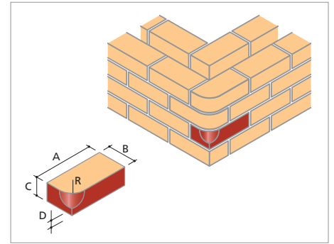
BN.3 Single Bullnose Stop (Left & Right Hand)
