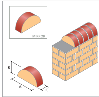
CP.1.2 Half Round Copping
