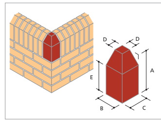
SD.3 Soldier External Return To Single Cant On End*
