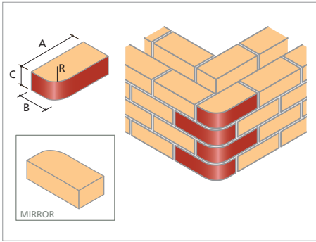
BN.1 Single Bullnose (Left & Right Hand)
